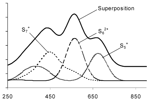
Figure 7. Simulated 71 UV-vis spectrum of “S 10.5 2+ ” including the contributions of the constituting S 6 2+ , S 5 + , and S 7 + ions approximately resembling the experimental spectrum given 70 as S 8 2+ (trace B) in Figure 2 7 in the 400–800 nm region.
